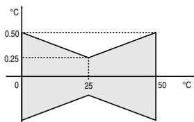
Temper. measurement (NTC res.), range 0...50°C
